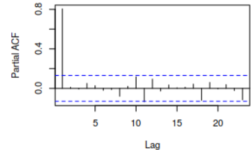
Series diff(c)
