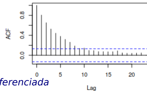
Series diff(c)
