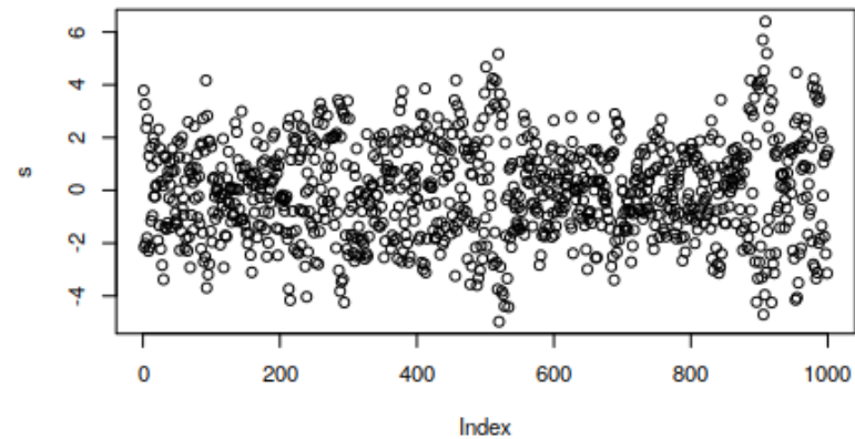
Series s
