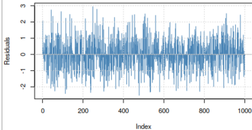
Standardized Residuals
