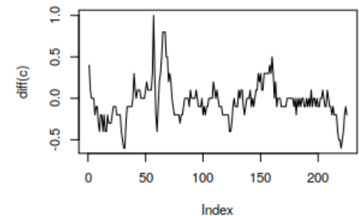
Series diff(c)
