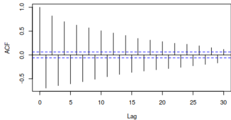
Series s
