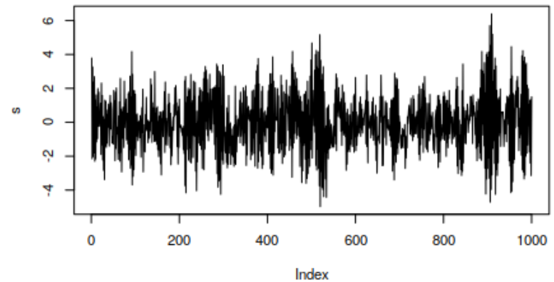
Series s
