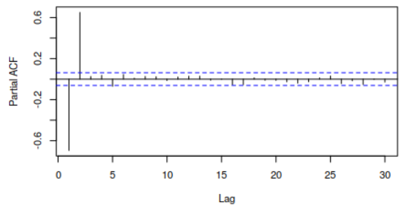
Series s
