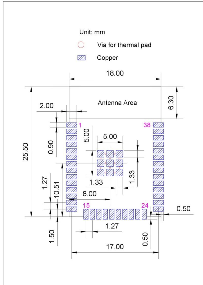
Figure 8: Recommended PCB Land Pattern
