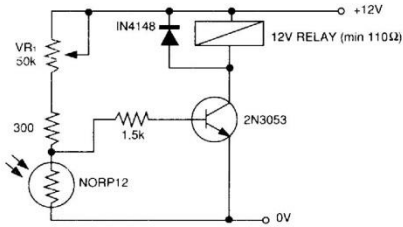
Figure 7 Light interruption detector
