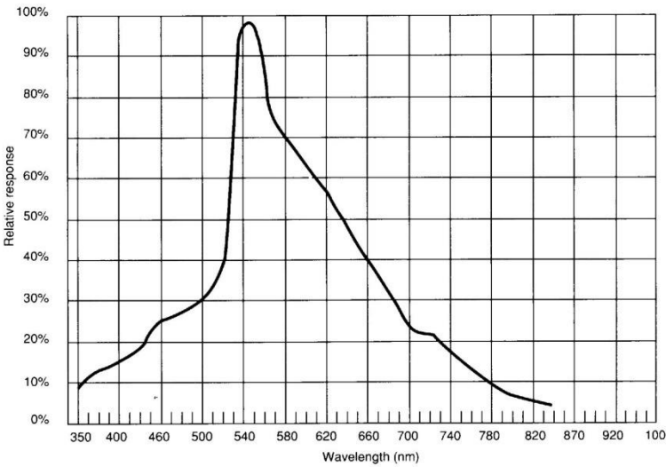
Figure 5 Spectral response
