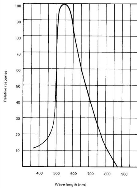
Figure 2 Spectral response
