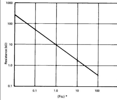
Figure 3 Resistance as a function of illumination
