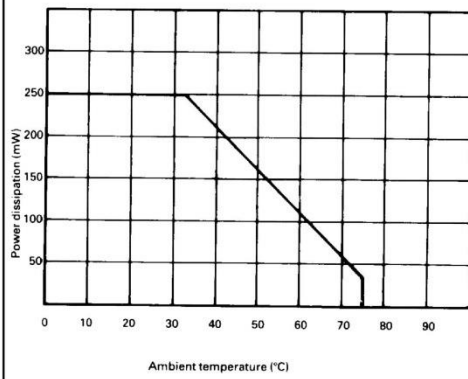
Figure 1 Power dissipation derating
