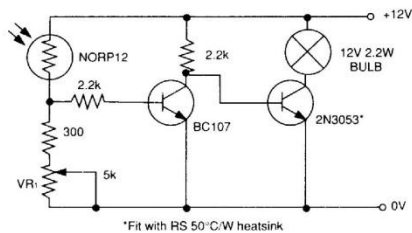
Figure 8 Automatic light circuit
