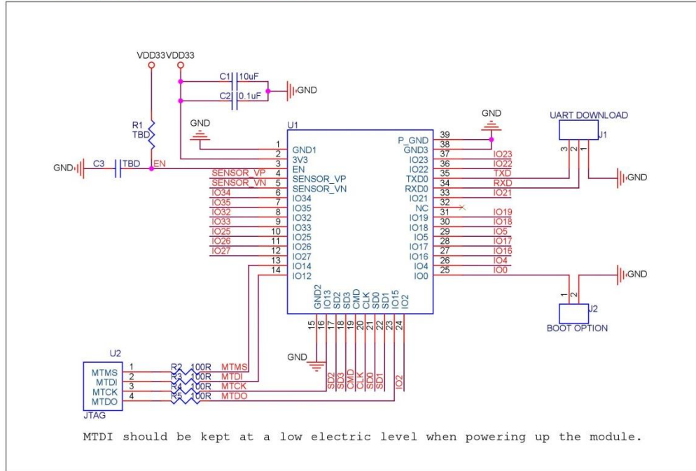
Figure 4: ESP32-WROOM-32 Peripheral Schematics
