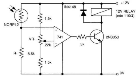
Figure 10 Extremely sensitive light operated relay
