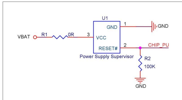
Figure 6: Reset Circuit
