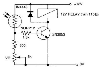
Figure 6 Sensitive light operated relay
