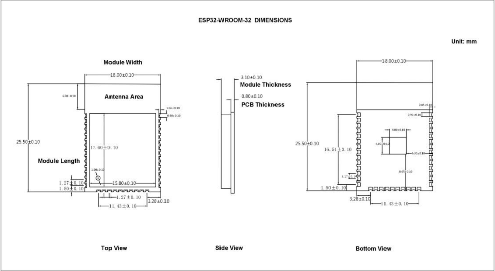
Figure 7: Physical Dimensions of ESP32-WROOM-32
