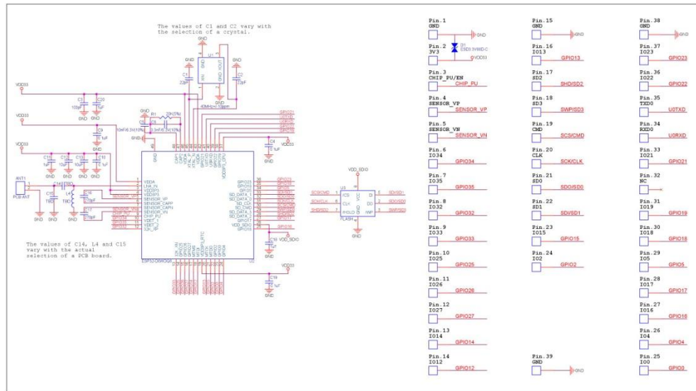
Figure 3: ESP32-WROOM-32 Schematics
