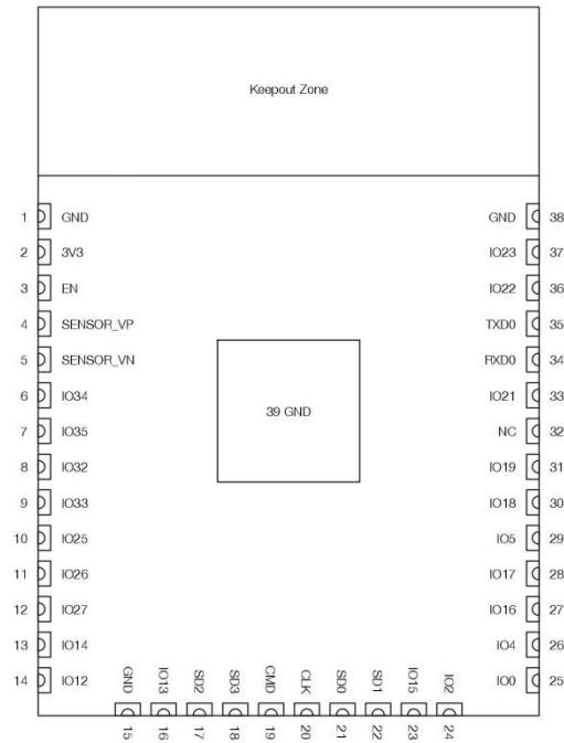
Figure 1: ESP32-WROOM-32 Pin Layout (Top View)
