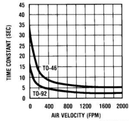
Thermal Time Constant
