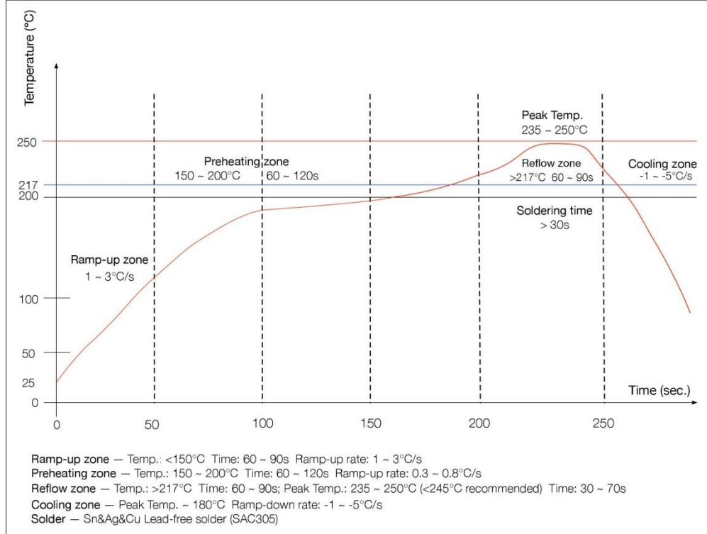
Figure 2: Reflow Profile
