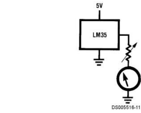
FIGURE 11. Centigrade Thermometer (Analog Meter)
