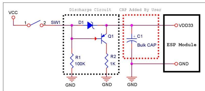
Figure 5: Discharge Circuit for VDD33 Rail
